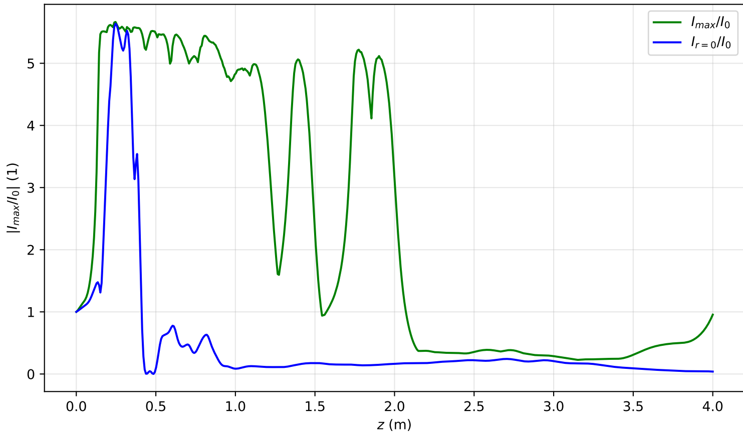
I_{max}(x = 0, y = 0, z)/I_0 , P_{in}=19.8\text{Pcr} , noisy input, artificial time
