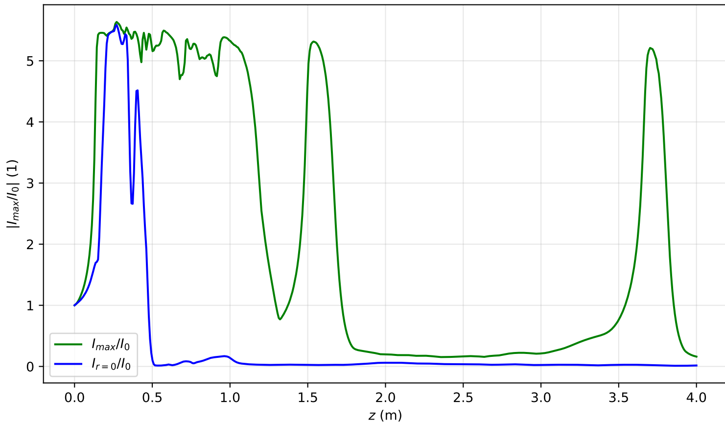
I_{\max}(x = 0, y = 0, z)/I_0 , Pin=19.9Pcr, noisy input, artificial time
