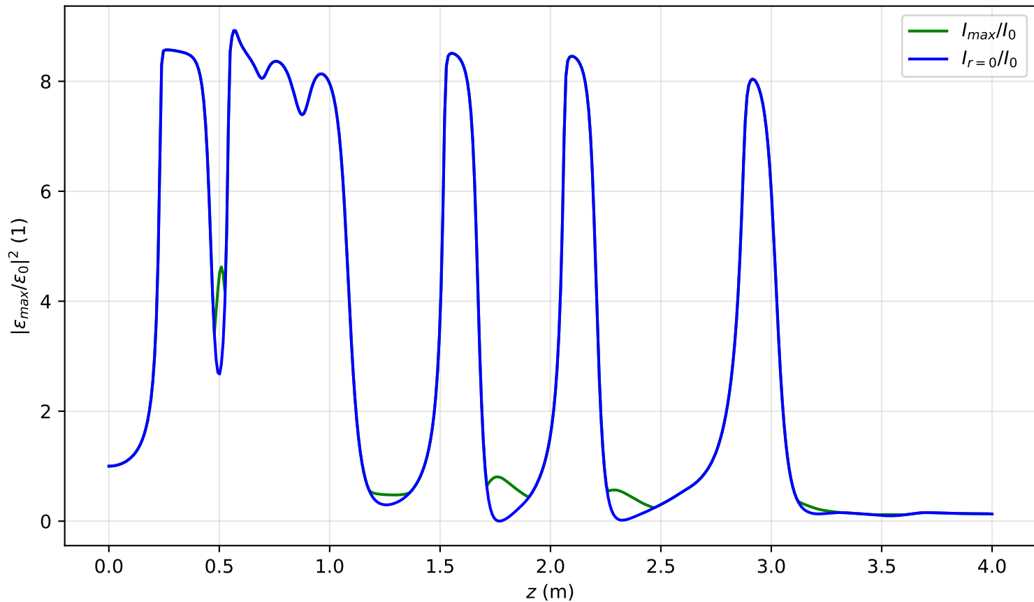
Max intensity over time vs z, artificial time
