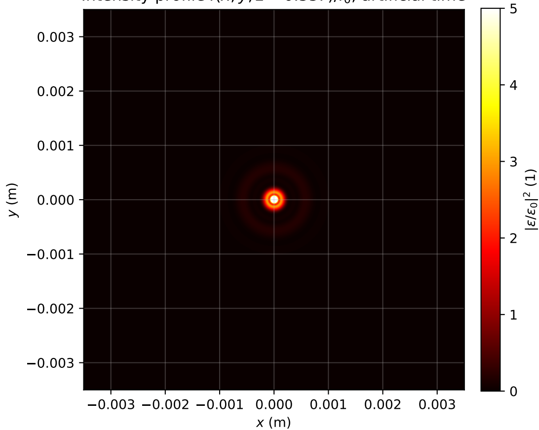
Intensity profile I(x, y, z = 0.557)/I_0 , artificial time
