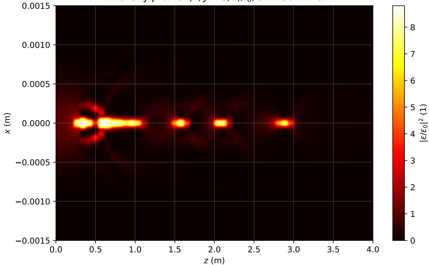
Intensity profile I(x, y = 0, z)/I_0 , artificial time
