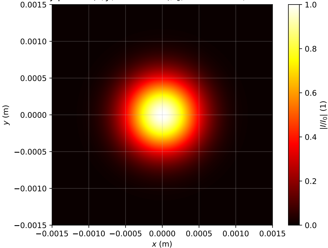
Intensity profile I(x, y, z = 0.000m)/I_0 , P_{in}=13.5P_{cr} , artificial time
