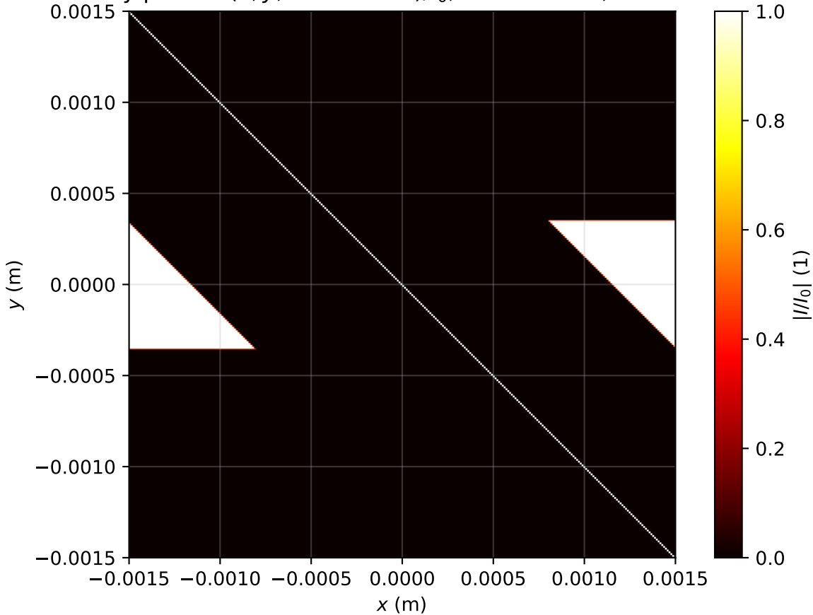
Intensity profile I(x, y, z = 0.000m)/I_0 , P_{in}=13.0P_{cr} , artificial time
