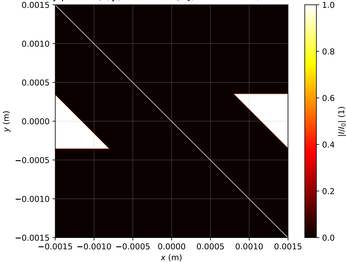
Intensity profile I(x, y, z = 0.000m)/I_0 , P_{in}=17.0P_{cr} , artificial time
