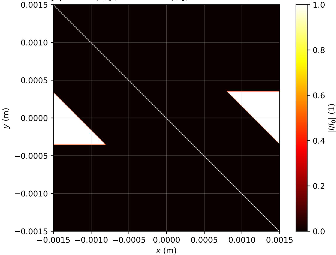
Intensity profile I(x, y, z = 0.000m)/I_0 , P_{in}=19.0P_{cr} , artificial time
