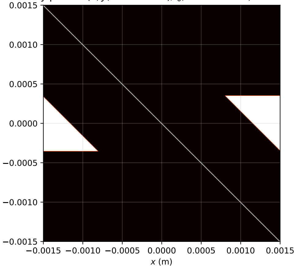
Intensity profile I(x, y, z = 0.000m)/I_0 , P_{in}=20.0P_{cr} , artificial time
