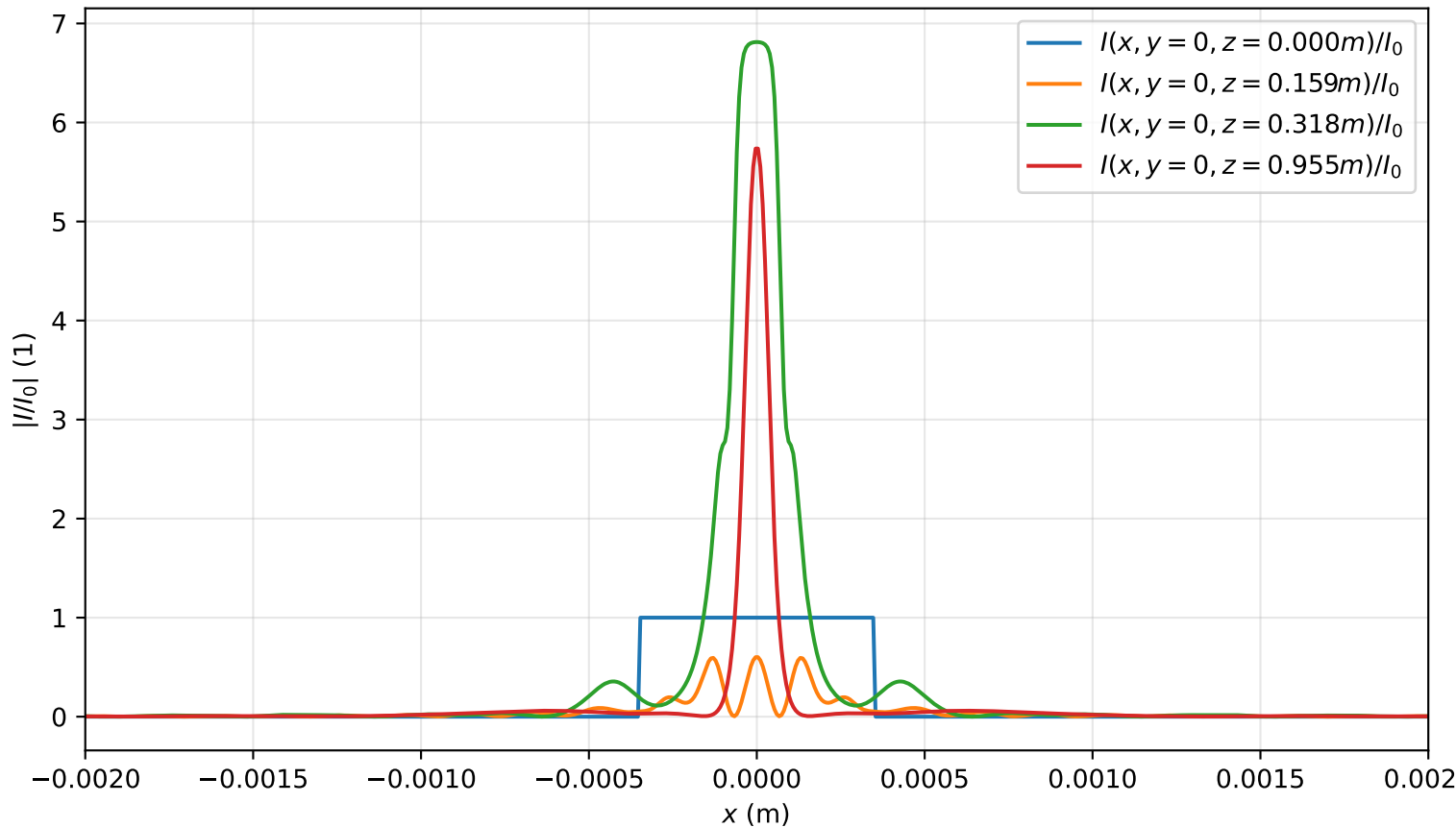
Intensity profile I(x, y = 0, z)/I_0 , P_{in}=11.0\text{Pcr} , artificial time
