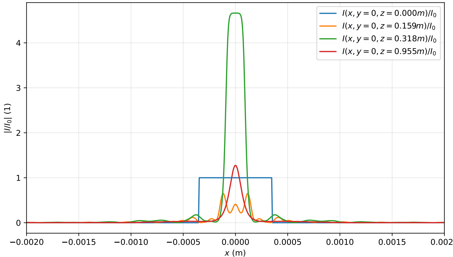
Intensity profile I(x, y = 0, z)/I_0 , P_{in}=15.0P_{cr} , artificial time
