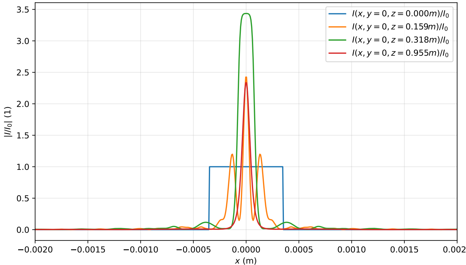
Intensity profile I(x, y = 0, z)/I_0 , \text{Pin}=20.0\text{Pcr} , artificial time
