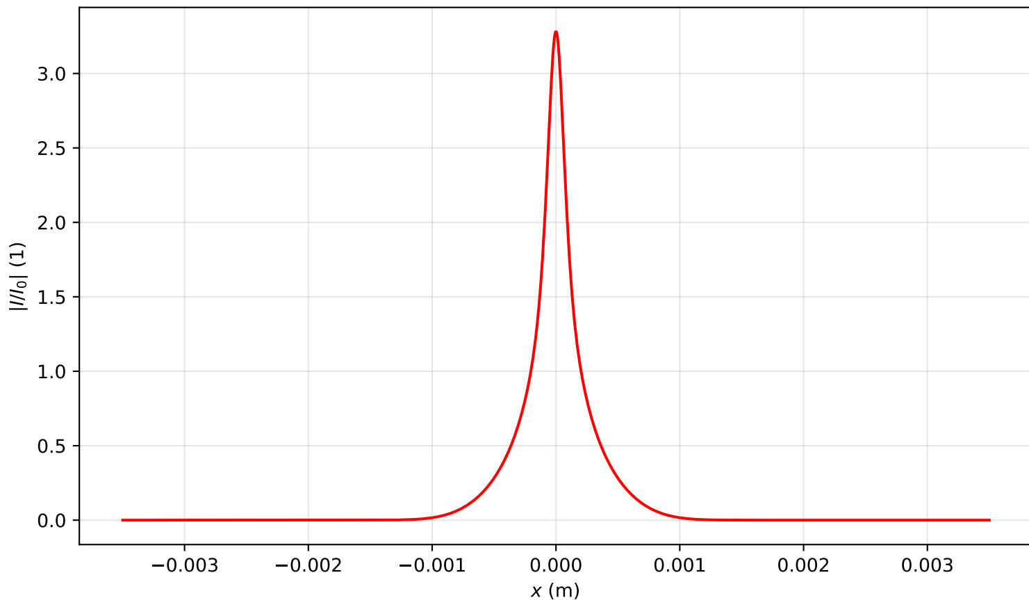
Intensity profile I(x, y = 0, z = 0.239)/I_0 , P_{in}=10.5P_{cr} , artificial time
