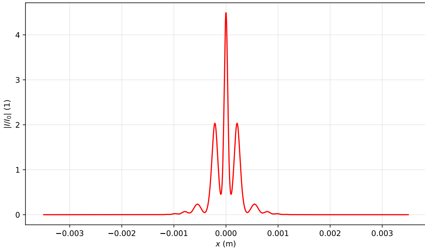
Intensity profile I(x, y = 0, z = 0.478)/I_0 , P_{in}=10.5P_{cr} , artificial time
