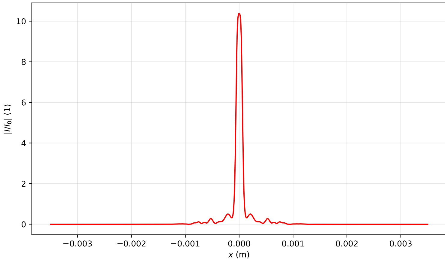
Intensity profile I(x, y = 0, z = 0.716)/I_0 , P_{in}=10.5P_{cr} , artificial time
