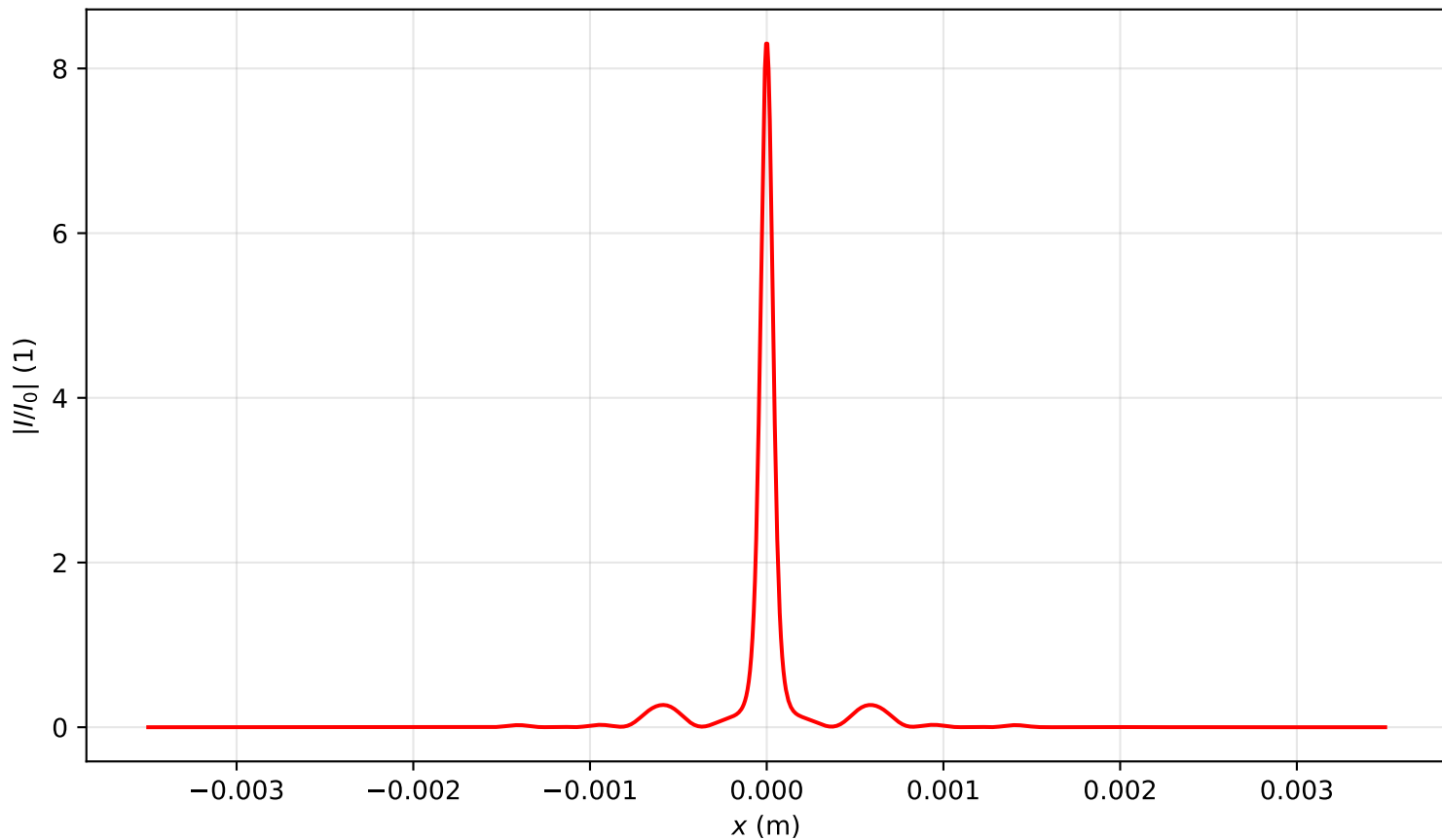
Intensity profile I(x, y = 0, z = 0.955)/I_0 , P_{in}=10.5P_{cr} , artificial time
