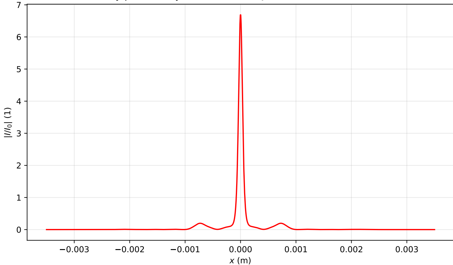
Intensity profile I(x, y = 0, z = 1.194)/I_0 , P_{in}=10.5P_{cr} , artificial time
