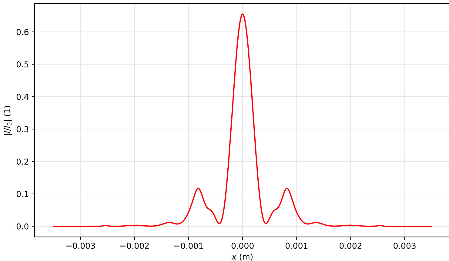
Intensity profile I(x, y = 0, z = 1.433)/I_0 , P_{in}=10.5P_{cr} , artificial time
