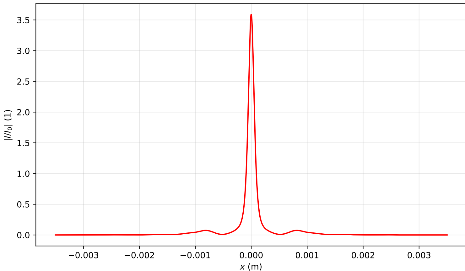
Intensity profile I(x, y = 0, z = 1.672)/I_0 , P_{in}=10.5P_{cr} , artificial time
