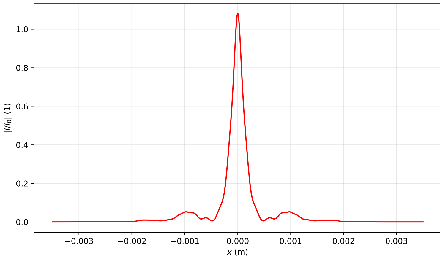
Intensity profile I(x, y = 0, z = 1.911)/I_0 , P_{in}=10.5P_{cr} , artificial time
