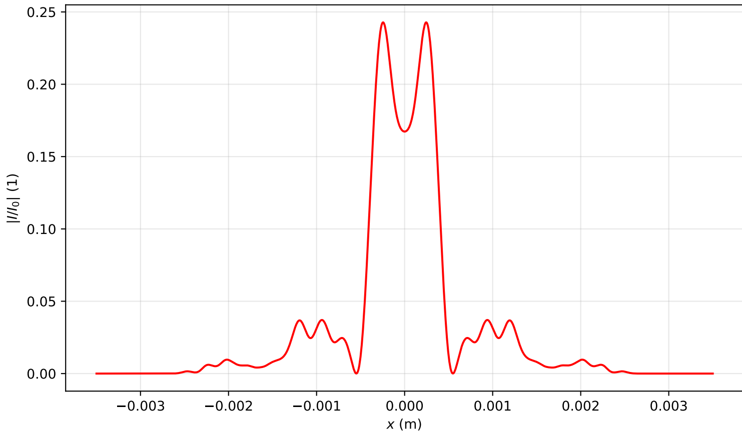
Intensity profile I(x, y = 0, z = 2.149)/I_0 , P_{in}=10.5P_{cr} , artificial time
