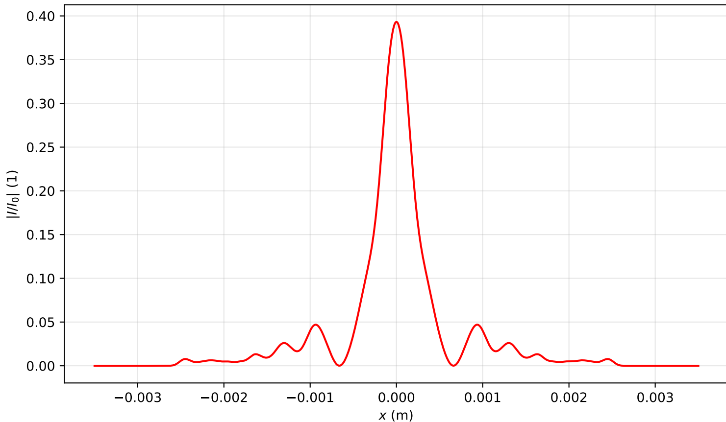
Intensity profile I(x, y = 0, z = 2.388)/I_0 , P_{in}=10.5P_{cr} , artificial time
