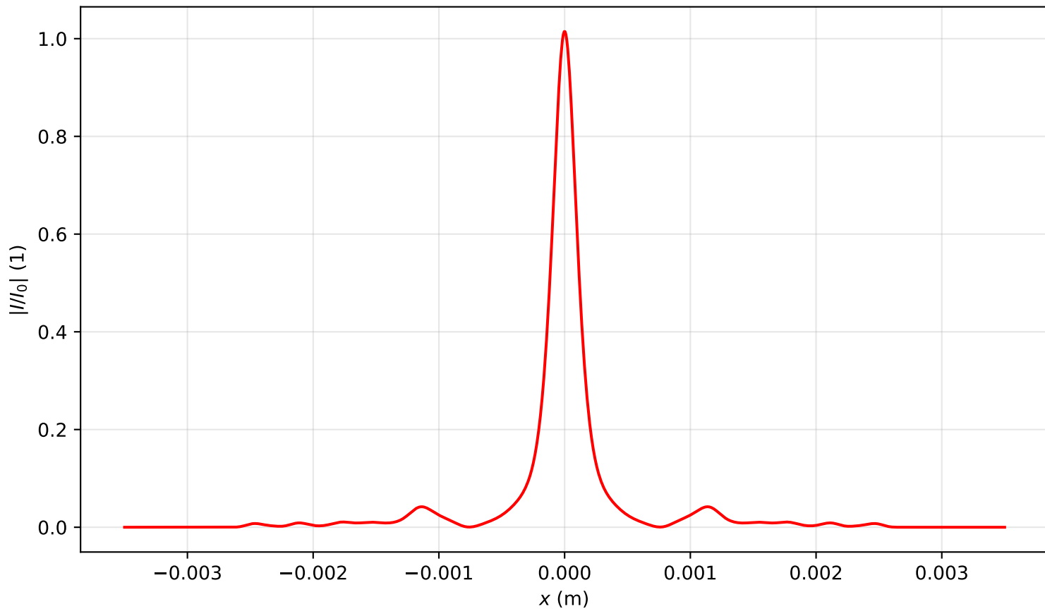
Intensity profile I(x, y = 0, z = 2.627)/I_0 , P_{in}=10.5P_{cr} , artificial time
