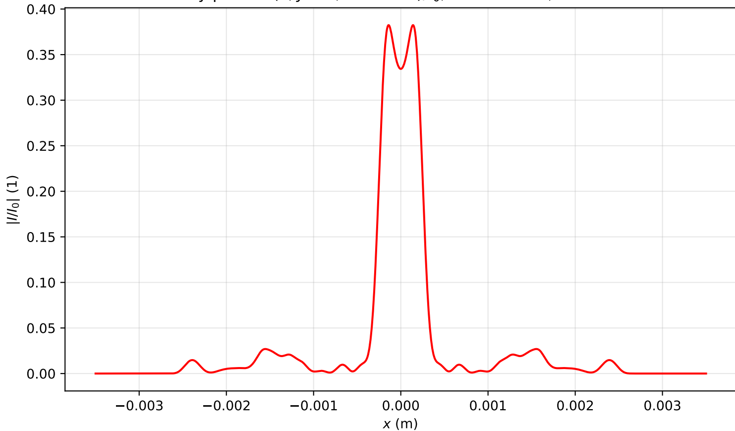
Intensity profile I(x, y = 0, z = 3.105)/I_0 , P_{in}=10.5P_{cr} , artificial time
