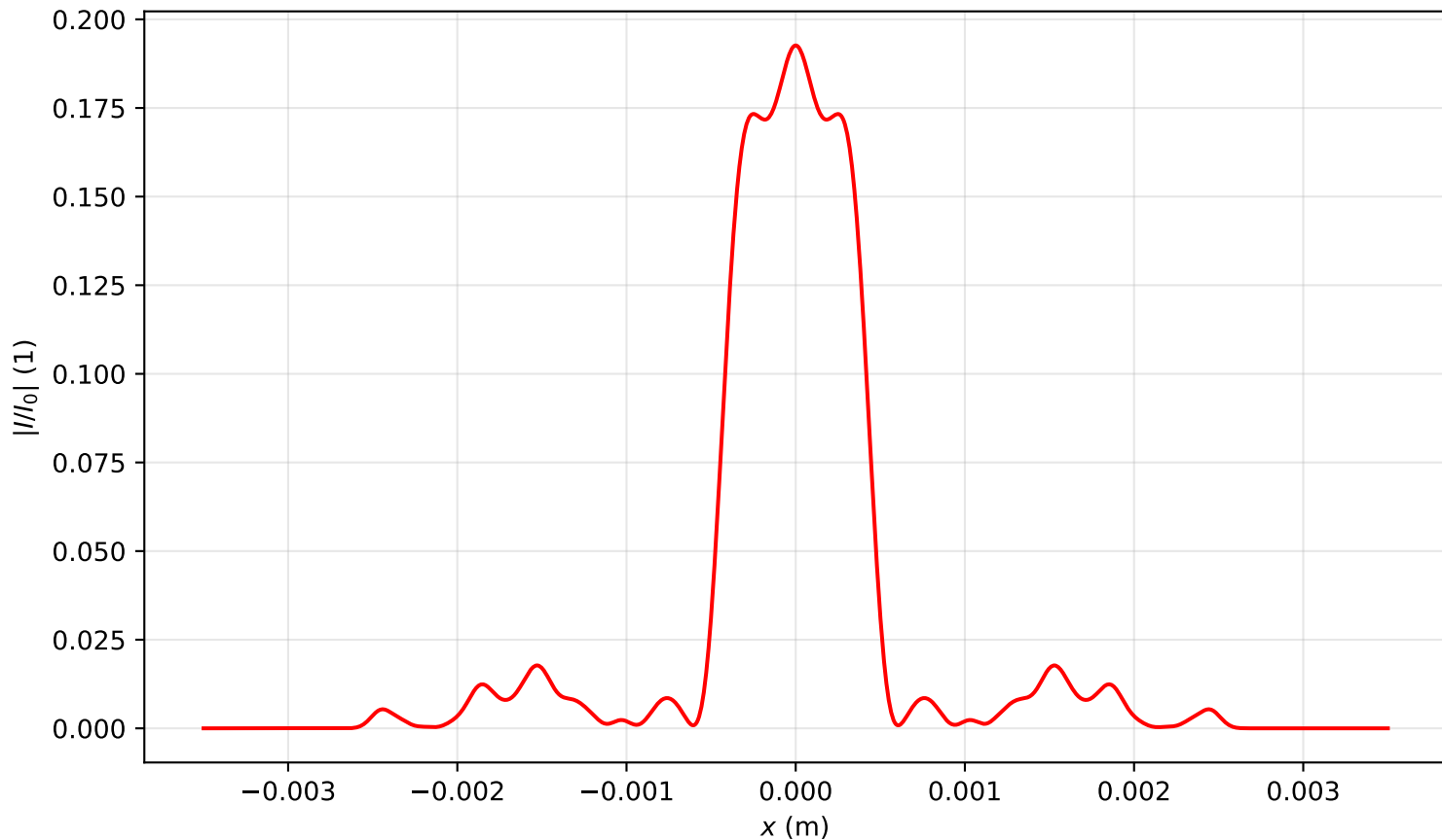
Intensity profile I(x, y = 0, z = 3.344)/I_0 , P_{in}=10.5P_{cr} , artificial time
