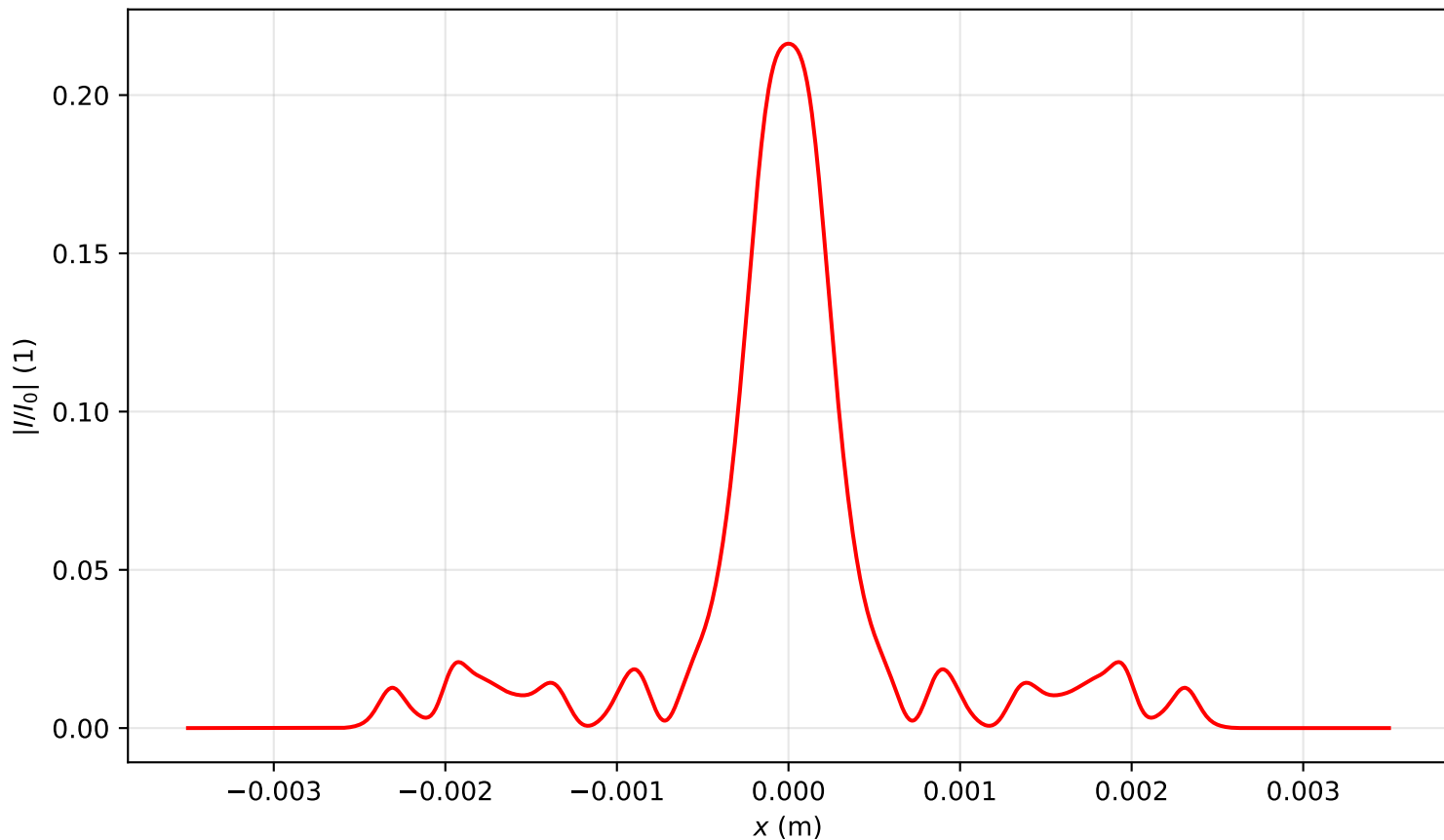
Intensity profile I(x, y = 0, z = 3.582)/I_0 , P_{in}=10.5P_{cr} , artificial time
