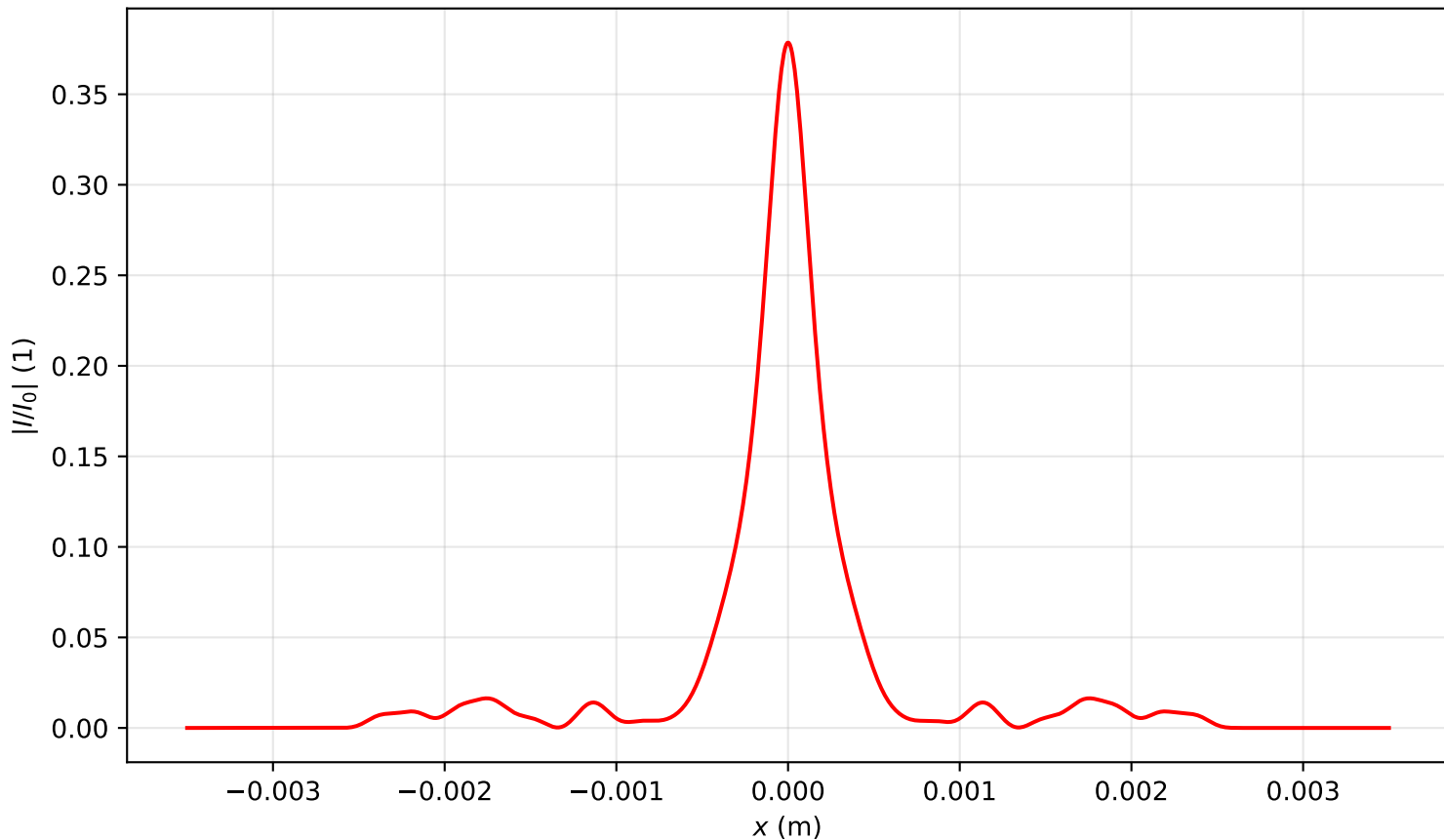
Intensity profile I(x, y = 0, z = 3.821)/I_0 , P_{in}=10.5P_{cr} , artificial time
