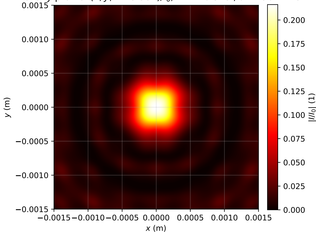
Intensity profile I(x, y, z = 3.582)/I_0 , P_{in}=10.5P_{cr} , artificial time
