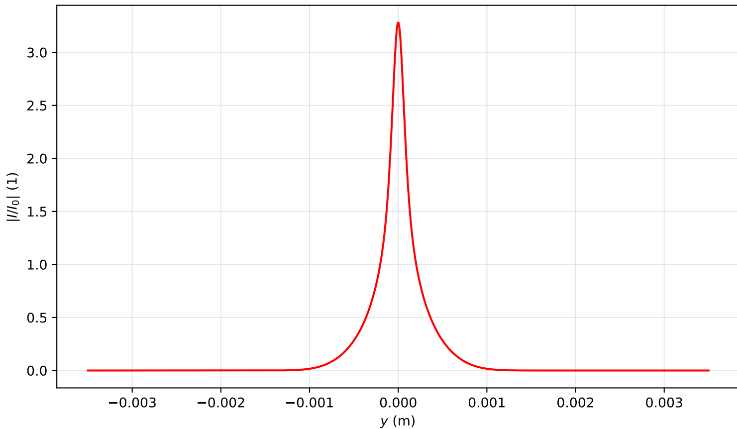
Intensity profile I(x=0, y, z=0.239)/I_0 , P_{in}=10.5P_{cr} , artificial time
