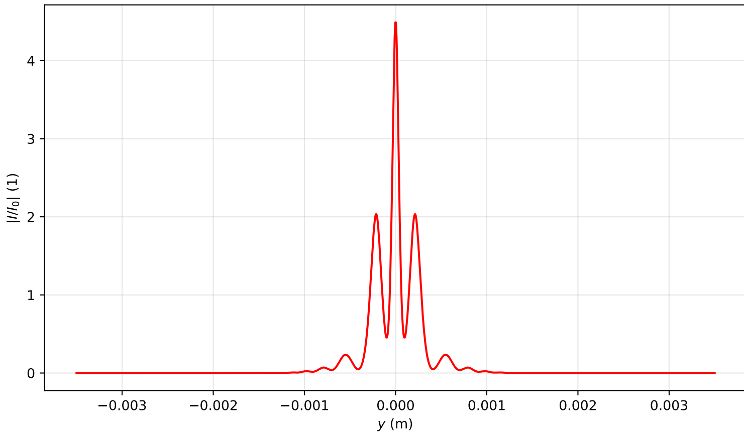
Intensity profile I(x=0, y, z=0.478)/I_0 , P_{in}=10.5P_{cr} , artificial time
