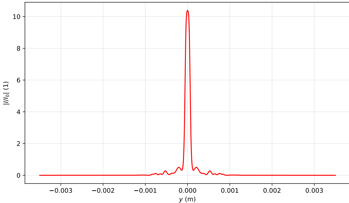
Intensity profile I(x=0, y, z=0.716)/I_0 , P_{in}=10.5P_{cr} , artificial time
