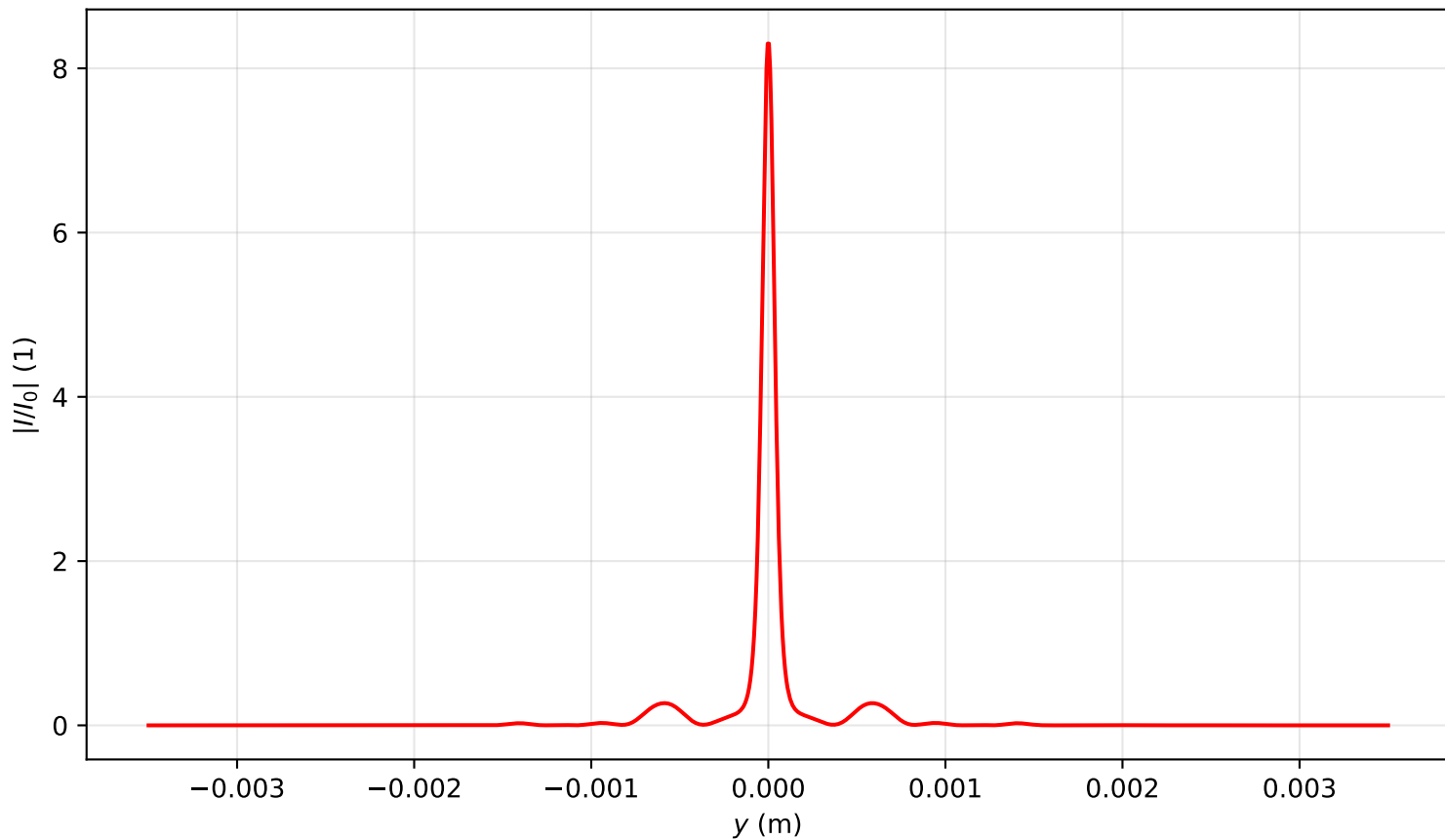
Intensity profile I(x=0, y, z=0.955)/I_0 , P_{in}=10.5P_{cr} , artificial time
