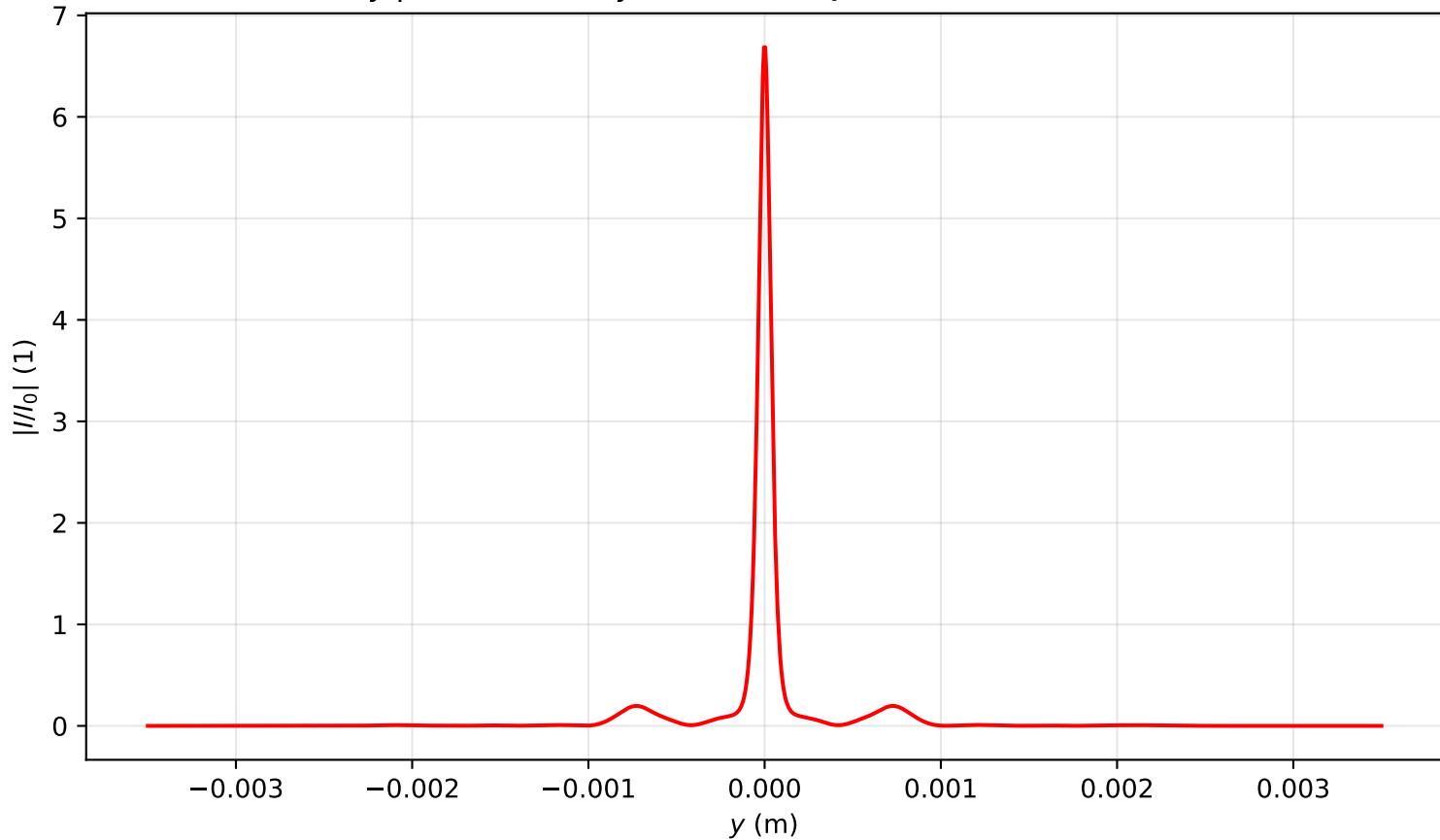
Intensity profile I(x=0, y, z=1.194)/I_0 , P_{in}=10.5P_{cr} , artificial time
