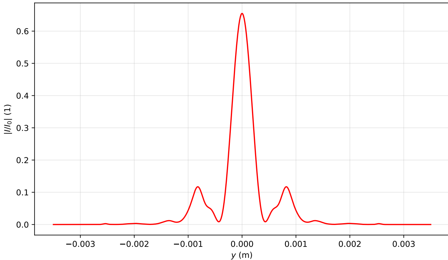
Intensity profile I(x=0, y, z=1.433)/I_0 , P_{in}=10.5P_{cr} , artificial time
