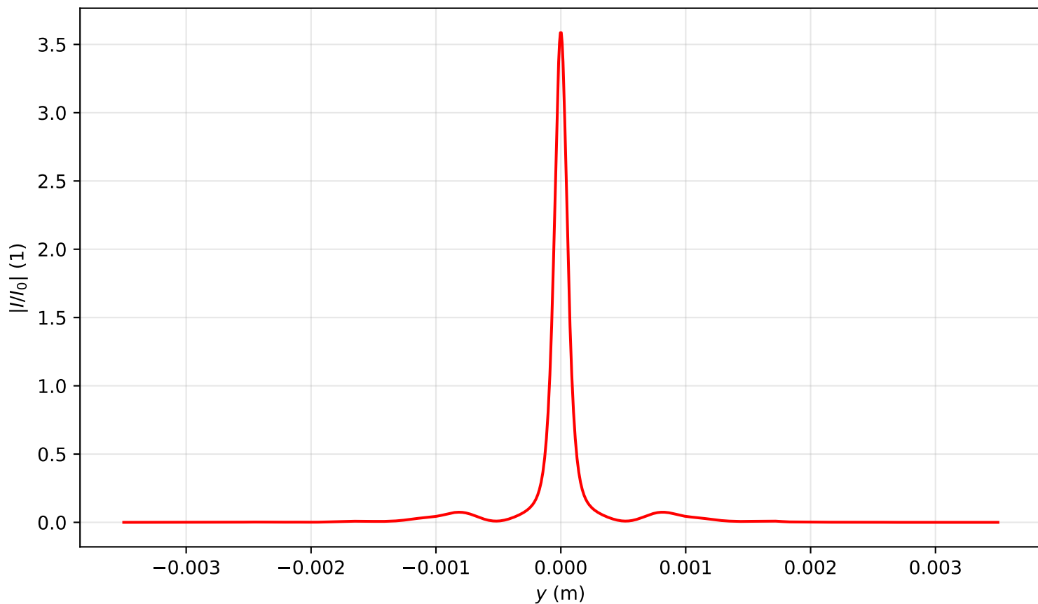
Intensity profile I(x=0, y, z=1.672)/I_0 , P_{in}=10.5P_{cr} , artificial time
