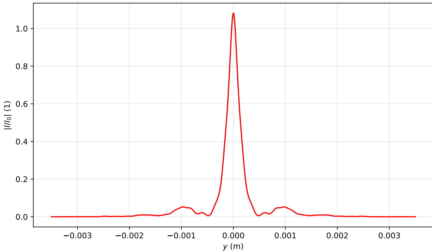
Intensity profile I(x=0, y, z=1.911)/I_0 , P_{in}=10.5P_{cr} , artificial time
