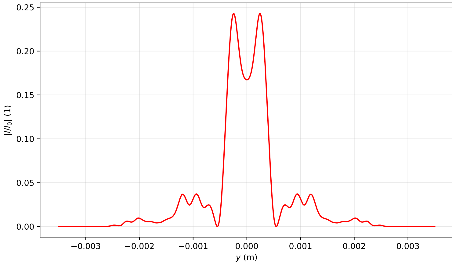
Intensity profile I(x = 0, y, z = 2.149)/I_0 , P_{in}=10.5P_{cr} , artificial time
