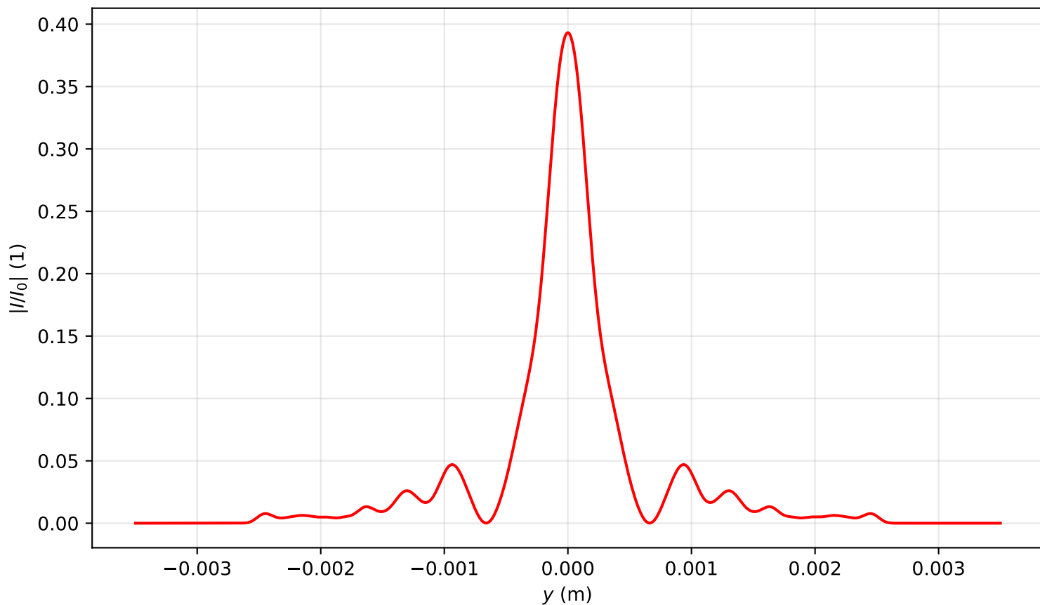
Intensity profile I(x=0, y, z=2.388)/I_0 , P_{in}=10.5P_{cr} , artificial time
