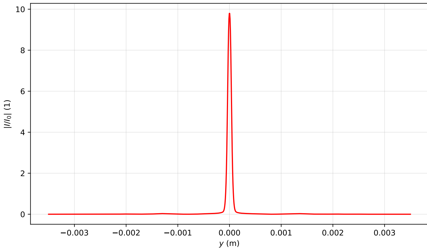
Intensity profile I(x=0, y, z=2.866)/I_0 , P_{in}=10.5P_{cr} , artificial time
