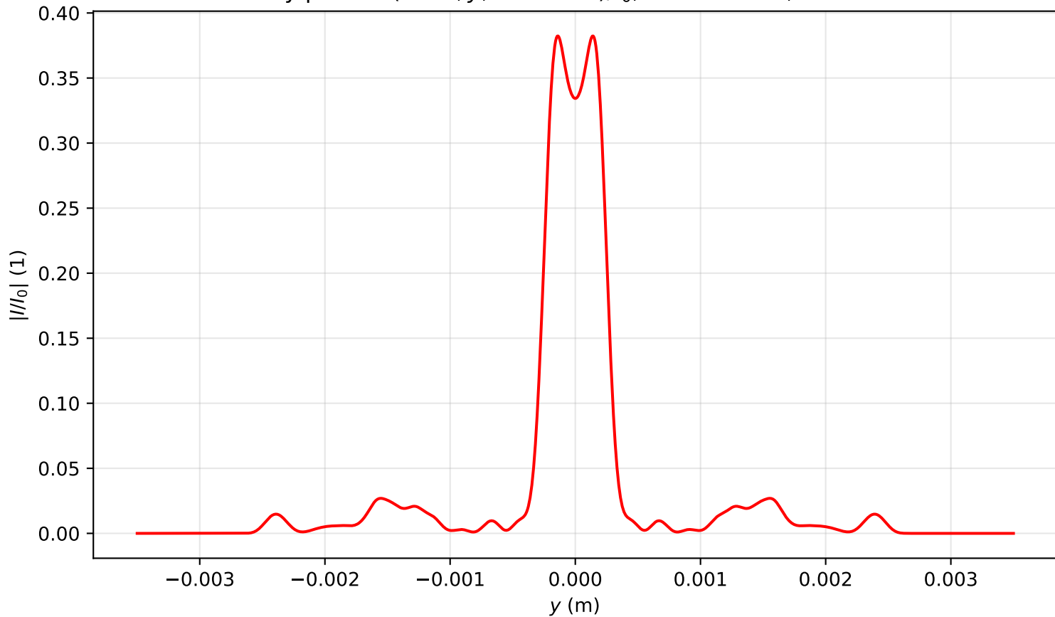
Intensity profile I(x=0, y, z=3.105)/I_0 , P_{in}=10.5P_{cr} , artificial time
