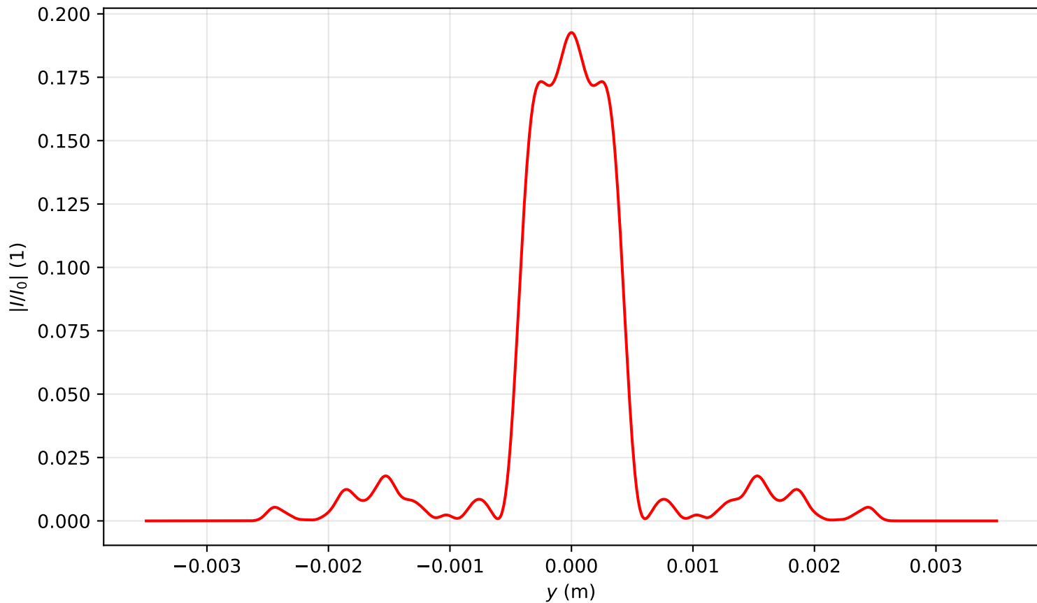
Intensity profile I(x=0, y, z=3.344)/I_0 , P_{in}=10.5P_{cr} , artificial time
