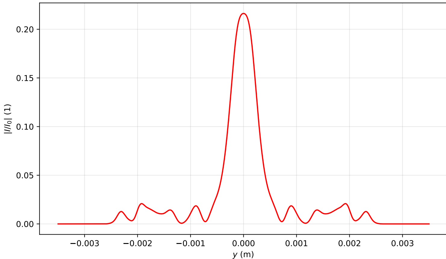
Intensity profile I(x = 0, y, z = 3.582)/I_0 , P_{in}=10.5P_{cr} , artificial time
