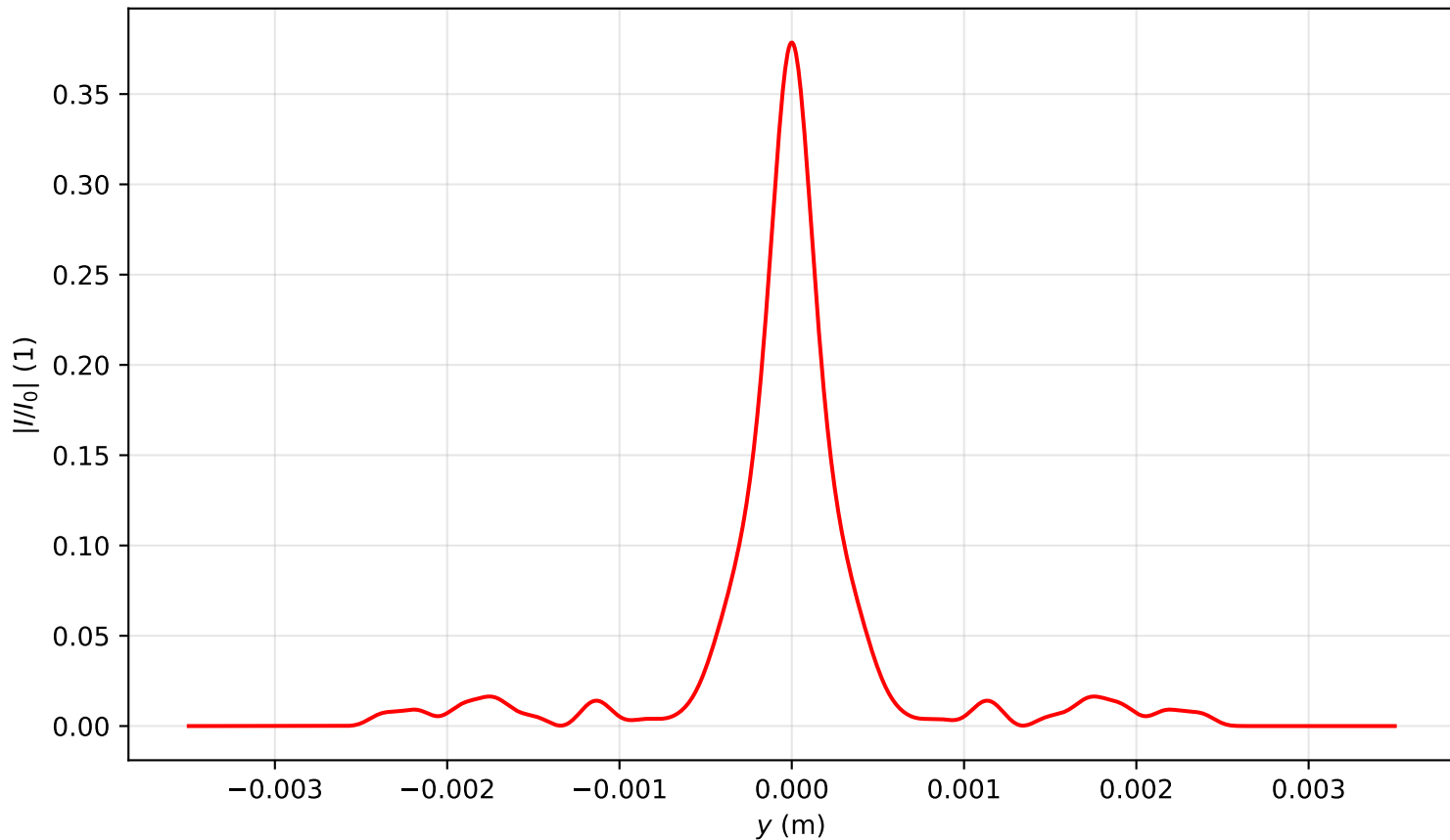
Intensity profile I(x=0, y, z=3.821)/I_0 , P_{in}=10.5P_{cr} , artificial time
