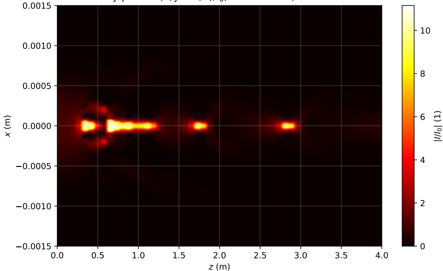
Intensity profile I(x, y = 0, z)/I_0 , P_{in}=10.5P_{cr} , artificial time
