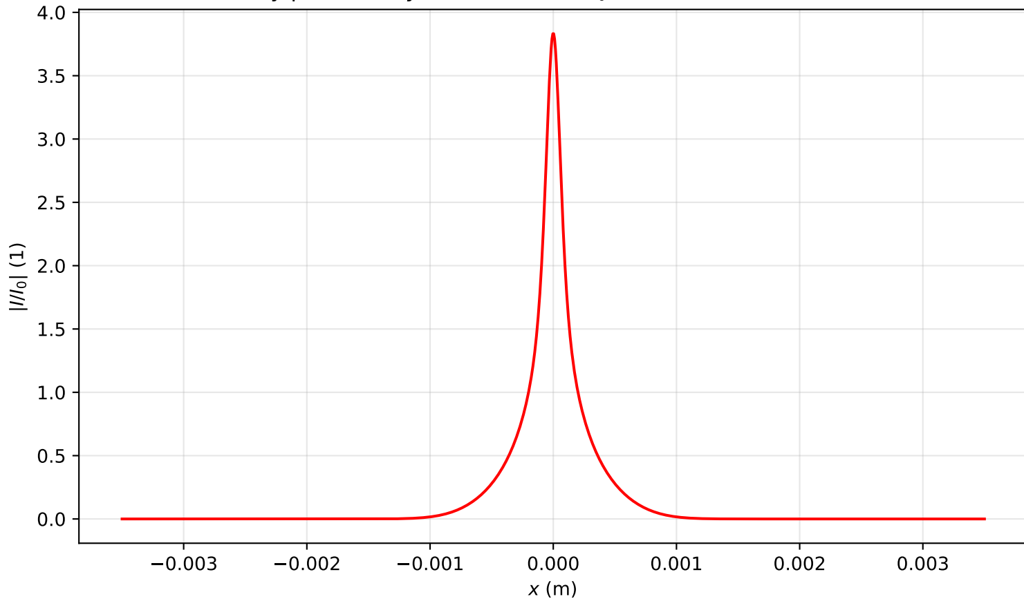
Intensity profile I(x, y = 0, z = 0.239)/I_0 , P_{in}=11.0P_{cr} , artificial time
