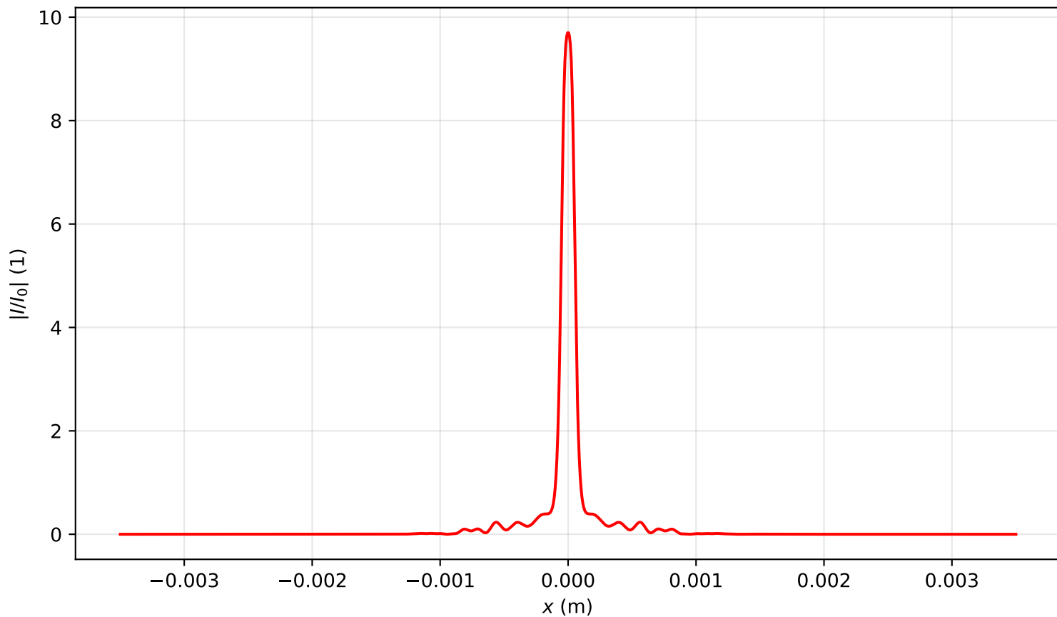
Intensity profile I(x, y = 0, z = 0.716)/I_0 , P_{in}=11.0P_{cr} , artificial time
