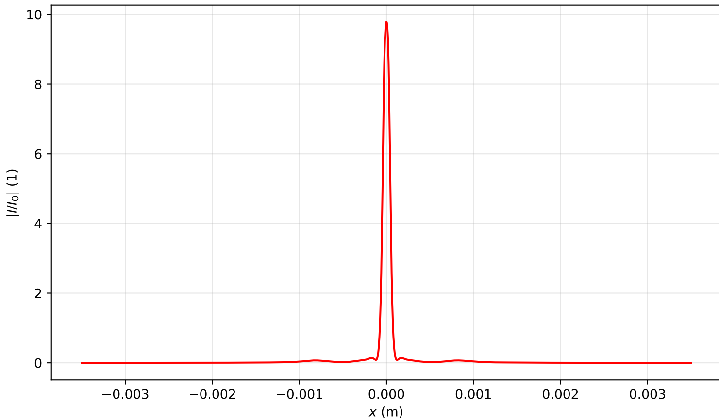
Intensity profile I(x, y = 0, z = 1.672)/I_0 , P_{in}=11.0P_{cr} , artificial time
