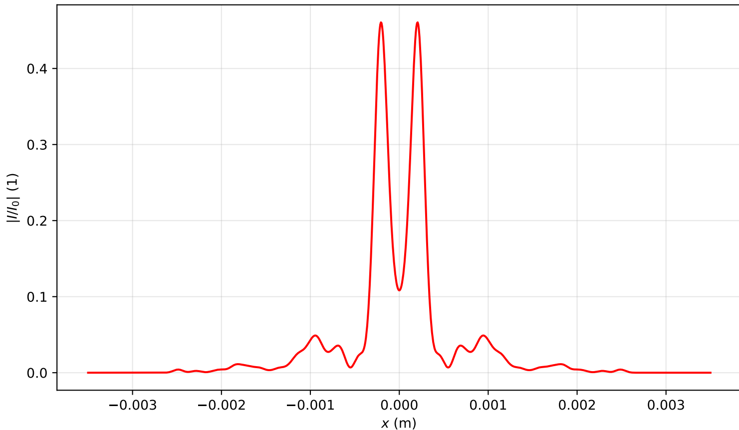
Intensity profile I(x, y = 0, z = 1.911)/I_0 , P_{in}=11.0P_{cr} , artificial time
