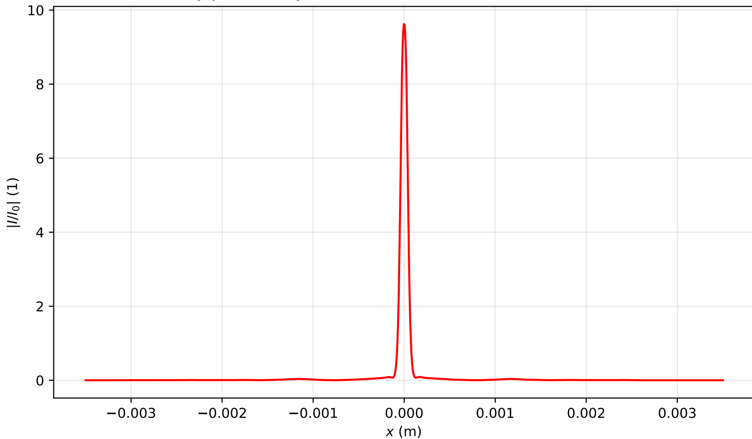
Intensity profile I(x, y = 0, z = 2.627)/I_0 , P_{in}=11.0P_{cr} , artificial time
